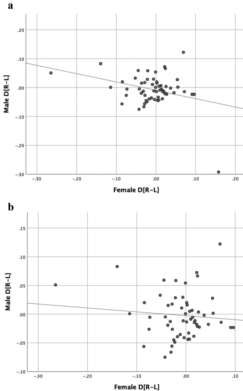
Fig. 1. Intra-couple correlation for D_{[R-L]} . Note. Fig. 1a presents the intra-couple correlation for D_{[R-L]} with all datapoints included ( r = -0.321, p = 0.014 ); Fig. 1b presents the same correlation with one outlier removed (the outlier in question is present in the bottom-right-hand corner of Fig. 1a ( r = -0.099, p = 0.465 )).
