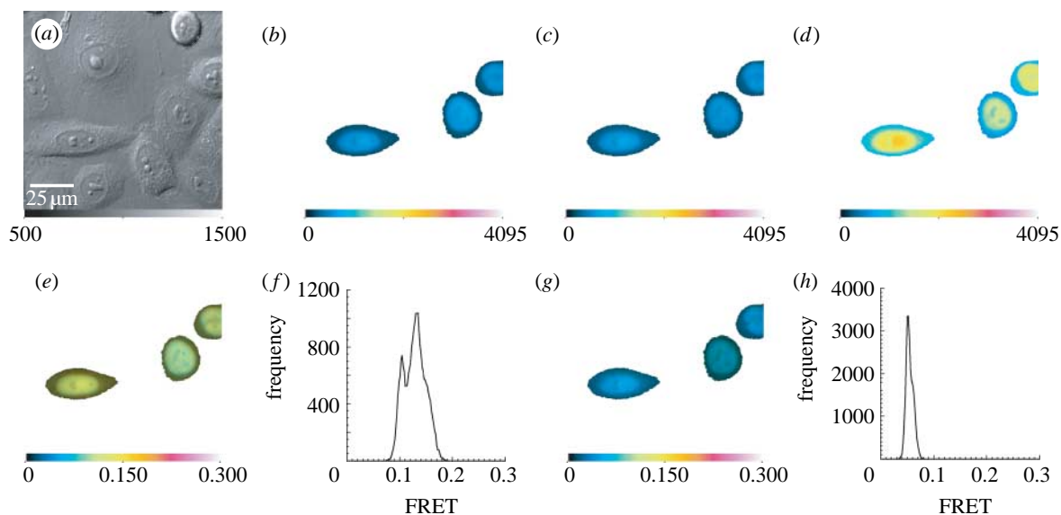
Figure 14. Intensity images and sensitized emission FRET analysis data for cyclin A tagged with cerulean and cdk1 tagged with EYFP. (a) Transmission image, (b) I^{\text{DD}} image, (c) I^{\text{DA}} image, (d) I^{\text{AA}} image, (e) intensity-overlay dFRET image, (f) dFRET histogram, (g) intensity-overlay aFRET image, (h) aFRET histogram.
